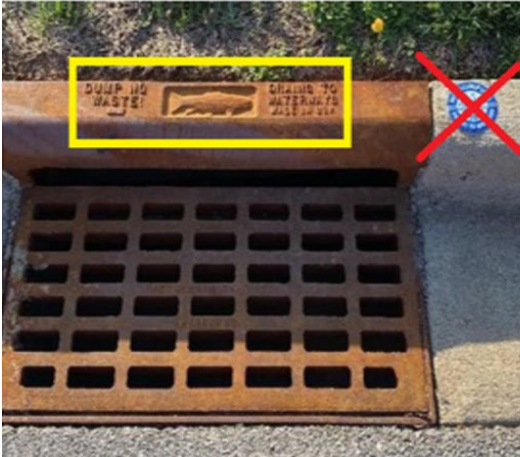
Figure 8: Storm drains with a permanent identifier (i.e. cast/lettered with “No Dumping, Drains to Stream/River”) should not be marked, they should be designated as Yes-Permanently Cast/Lettered
